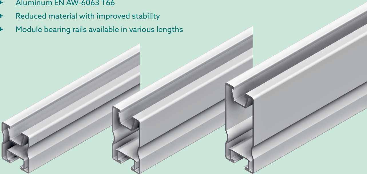
PROFILE PRO 35
